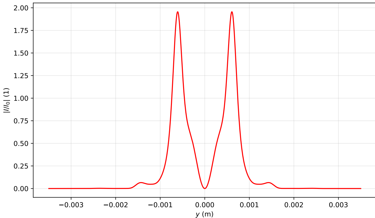
Intensity profile I(x=0, y, z=1.274)/I_0 , P_{in}=8.0P_{cr} , artificial time
